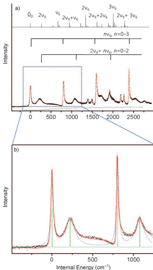
Figure 1. a) PHOFEX spectrum of diazirine with the simulation (red solid line) using the parameters listed in Table 1. Frank-Condon simulation with spectral assignments is shown above the spectrum while the \sigma' curve used in the Fano simulation is given beneath the spectrum (dotted line; see text for details). b) Extended view of the PHOFEX spectrum showing the simulation of the asymmetric rotor at T_{\text{rot}} = 10 K (green stick), the simulation convoluted by Lorentzians (blue dotted line), and Fano simulation (red solid line).
