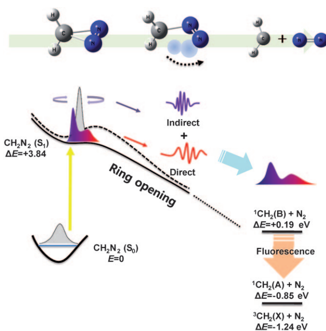
Figure 2. Schematic diagram showing the excitation of the bound and transition-state regions of the S_1 diazirine. The broken line represents a typical vibrational adiabatic surface showing a dynamic barrier, the nature of which depends on the extent of coupling to the reaction coordinate.
